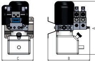
Montaggio verticale Vertical mounting
